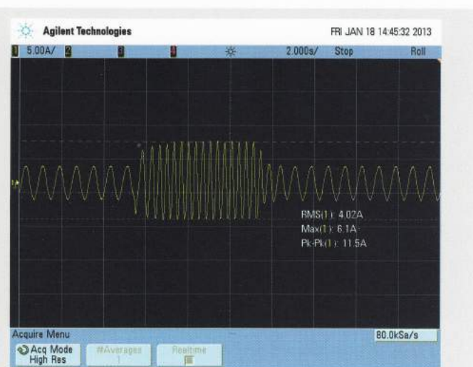
Current waveform in sudden acceleration/deceleration at 0.5Hz
